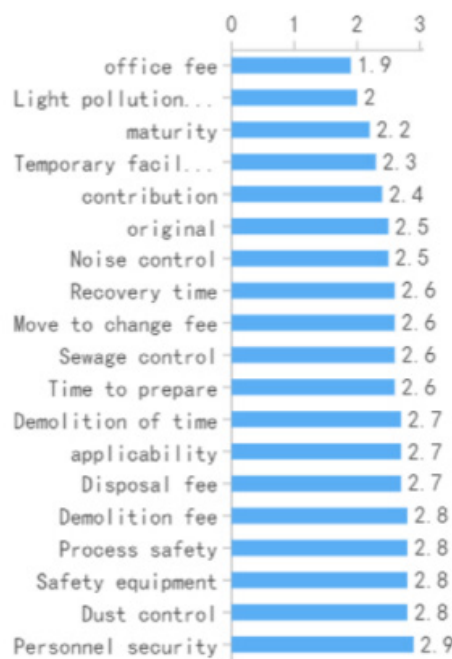
Figure. 1.Factorsaffecting the selectiong of urban overpass demolition scheme
