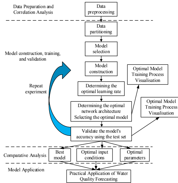
Figure 1: Technical Framework
